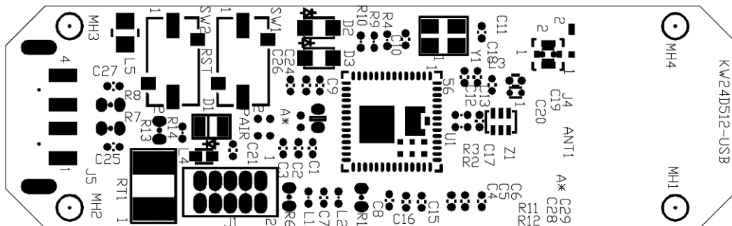
Figure 3-1. USB-KW24D512
