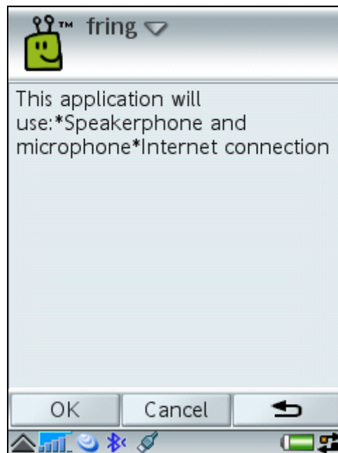
Figure 10- Confirmation Screen 1
