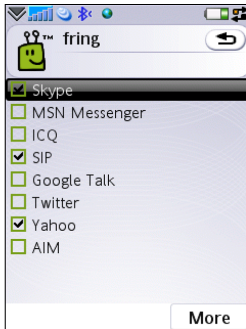
Figure 23 – Available services
