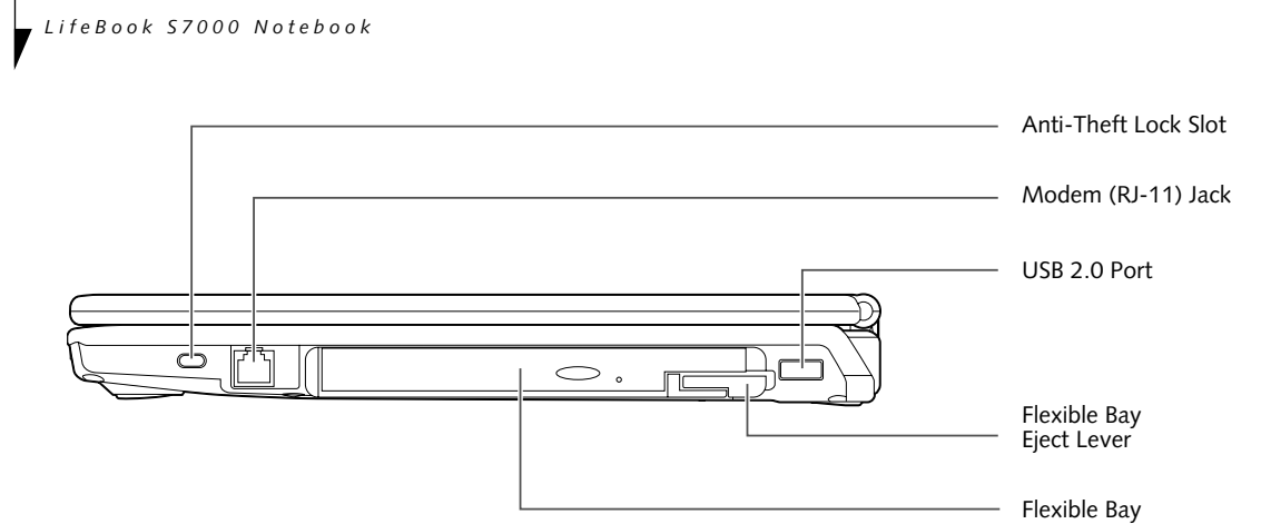
Figure 2-6. LifeBook notebook right-side panel
