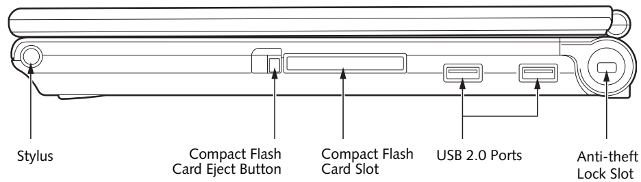
Figure 2-7. LifeBook notebook right-side panel
