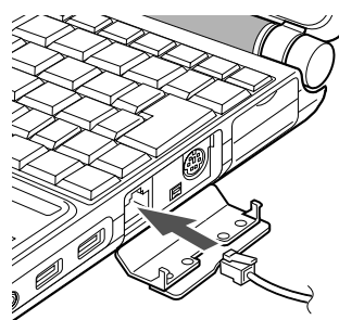
Figure 4-20 LAN Port
