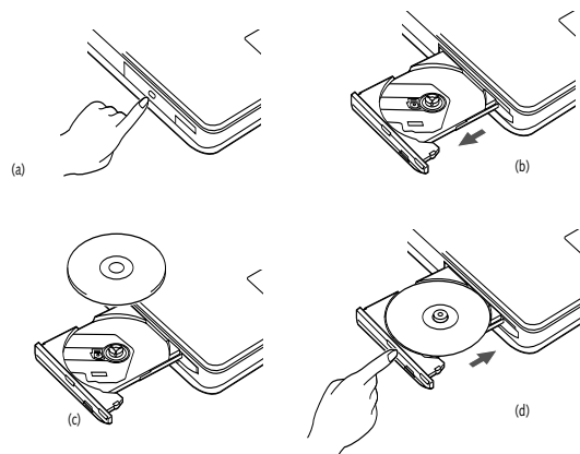
Figure 4-6 Loading/Removing Media
