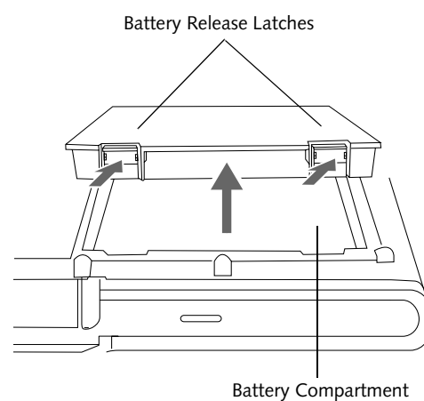
Figure 4-1. Removing the Battery
