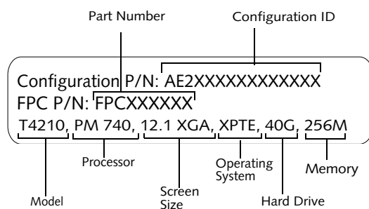
Figure 7-1. Configuration Label
