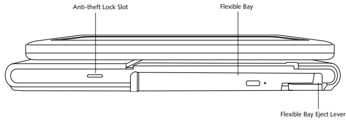
Figure 2-6. LifeBook T Series Tablet PC right-side panel
