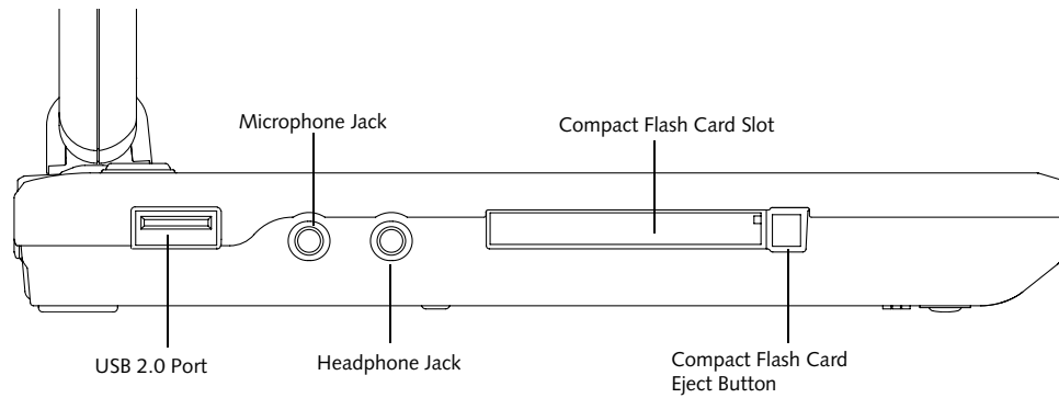
Figure 2-5. LifeBook P Series notebook/Tablet PC left-side panel
