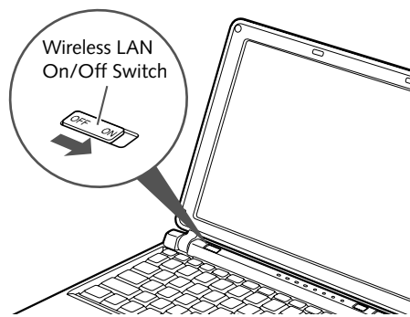
Figure 5-3. Wireless LAN On/Off Switch Location
