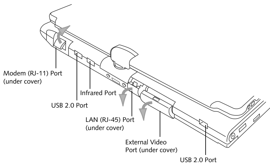
Figure 2-7. LifeBook T4200 Series Tablet PC rear panel
