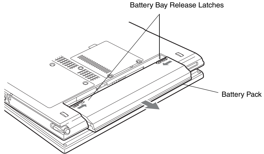
Figure 16. Removing a Battery
