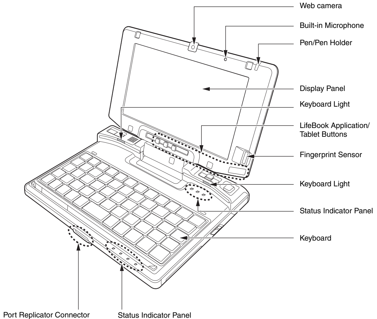
Figure 2. LifeBook U810 notebook in notebook mode
