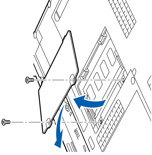
Figure 29. Opening the Memory Compartment
