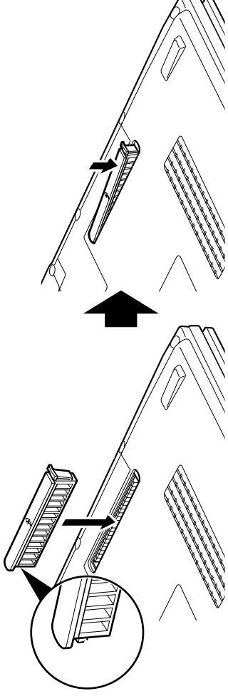
Figure 39. Removing/installing the dust filter
