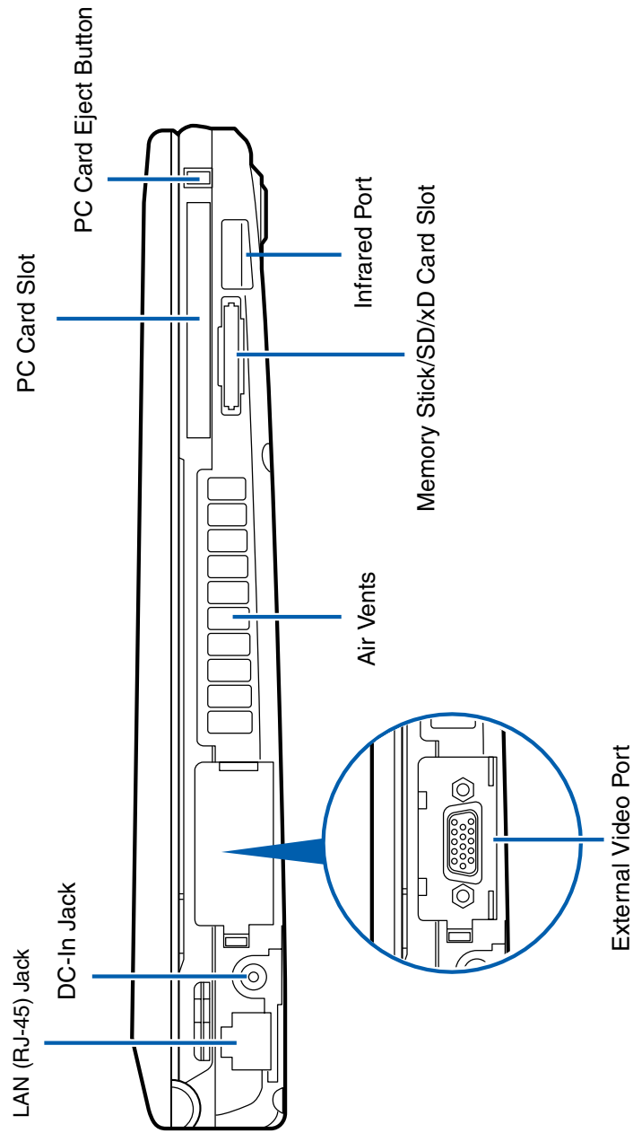
Figure 3. LifeBook notebook left-side panel
