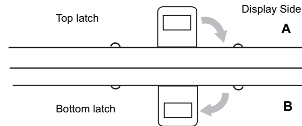
Figure 9. Latching/unlatching
