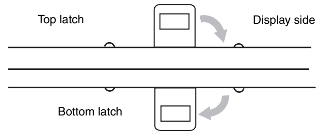
Figure 9. Latching/unlatching
