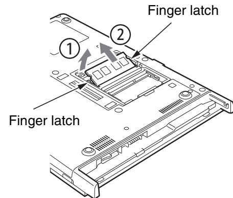
Figure 18. Removing a DIMM Module
