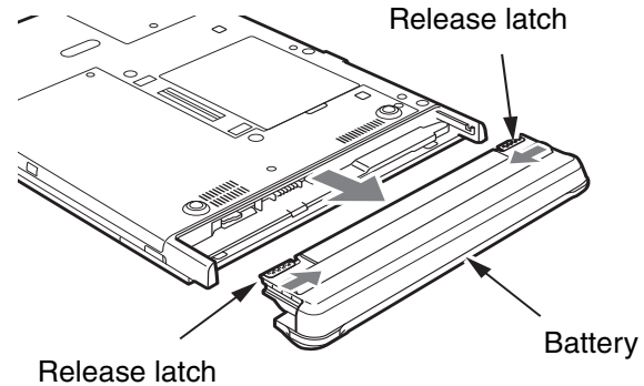
Figure 12. Removing the battery
