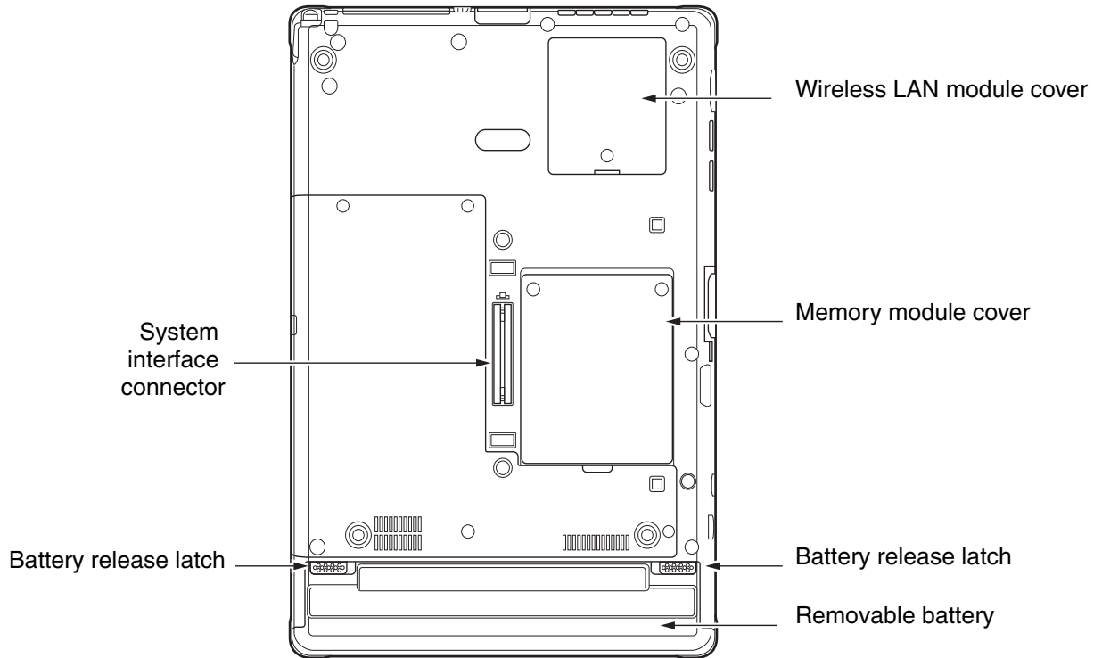
Figure 3. Stylistic ST6000 Series Tablet PC Features (Back View)
