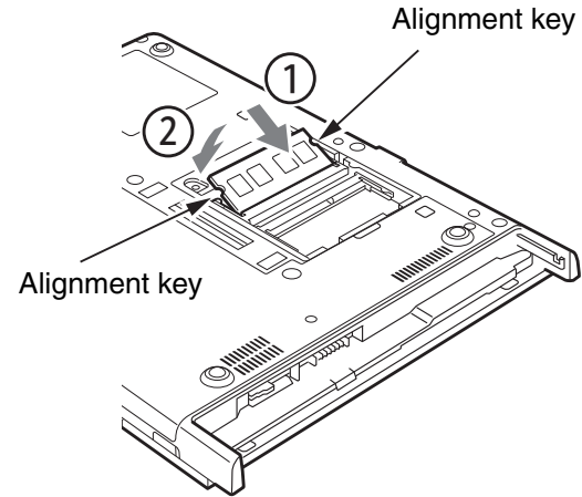
Figure 17. Installing a DIMM Module
