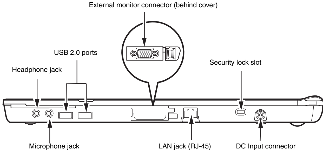
Figure 1-1. Stylistic ST6000 Series Tablet PC Features (Left Side View)
