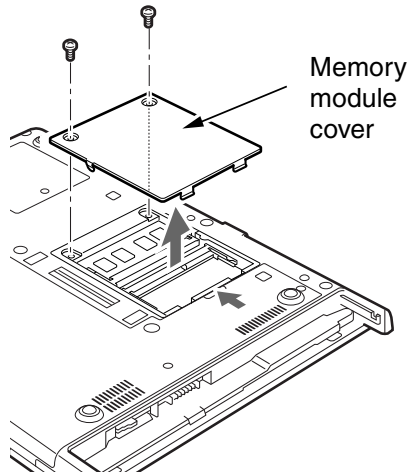
Figure 16. Accessing the Memory Slot
