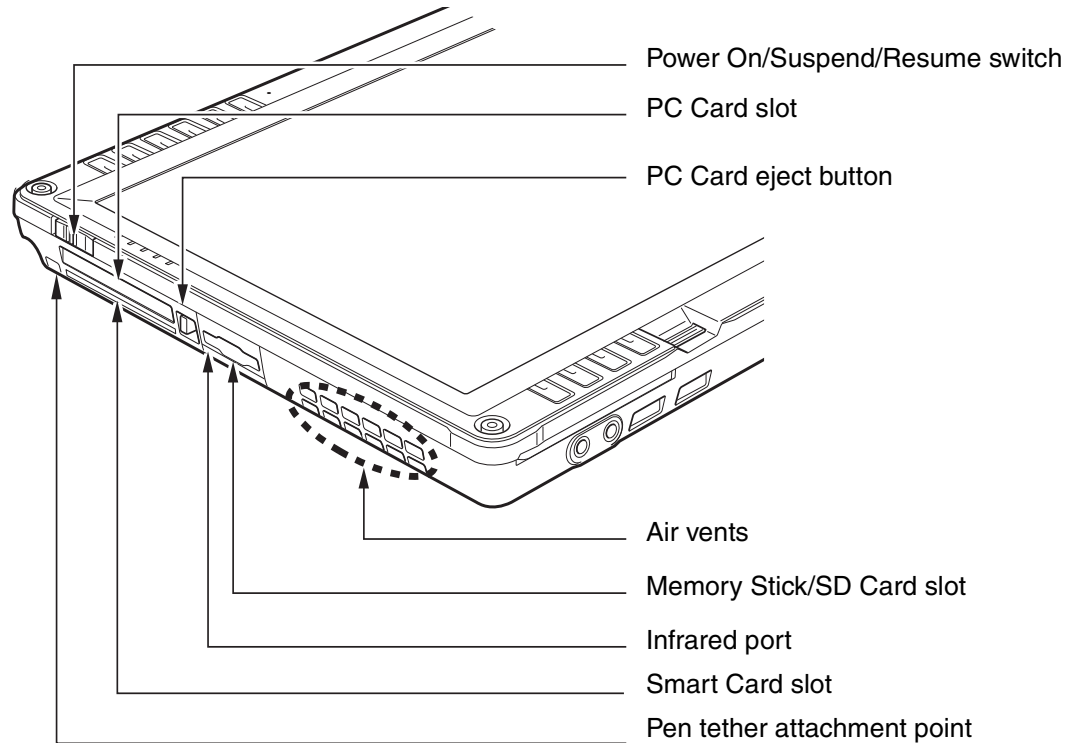
Figure 4. Stylistic ST6000 Series Tablet PC Features (Top View)
