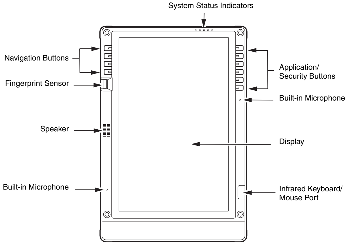
Figure 2. Stylistic ST6000 Series Tablet PC Features (Front View)
