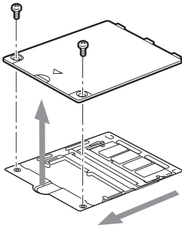
Figure 2-7. Accessing the Memory Slot
