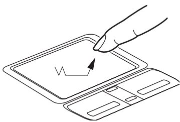
Figure 2-22. Dragging
