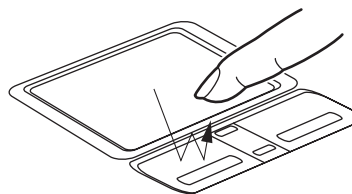
Figure 2-21. Double-clicking
