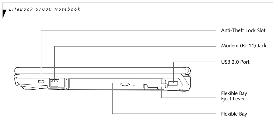
Figure 2-6. LifeBook notebook right-side panel
