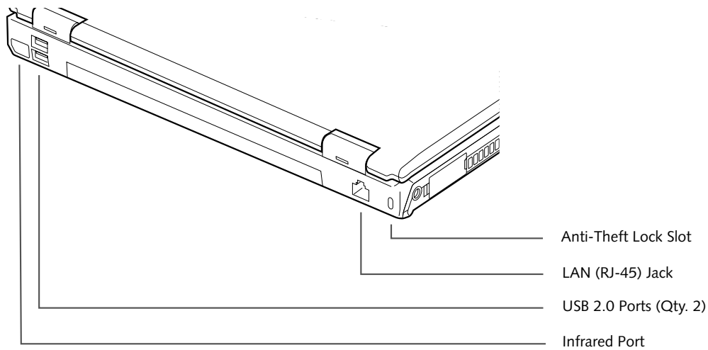
Figure 2-7. LifeBook notebook back panel
