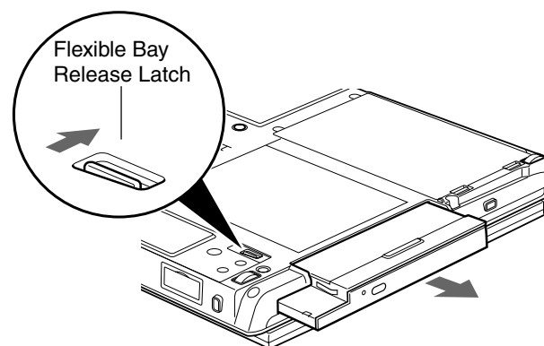
Figure 30. Removing/Installing Flexible Bay Device
