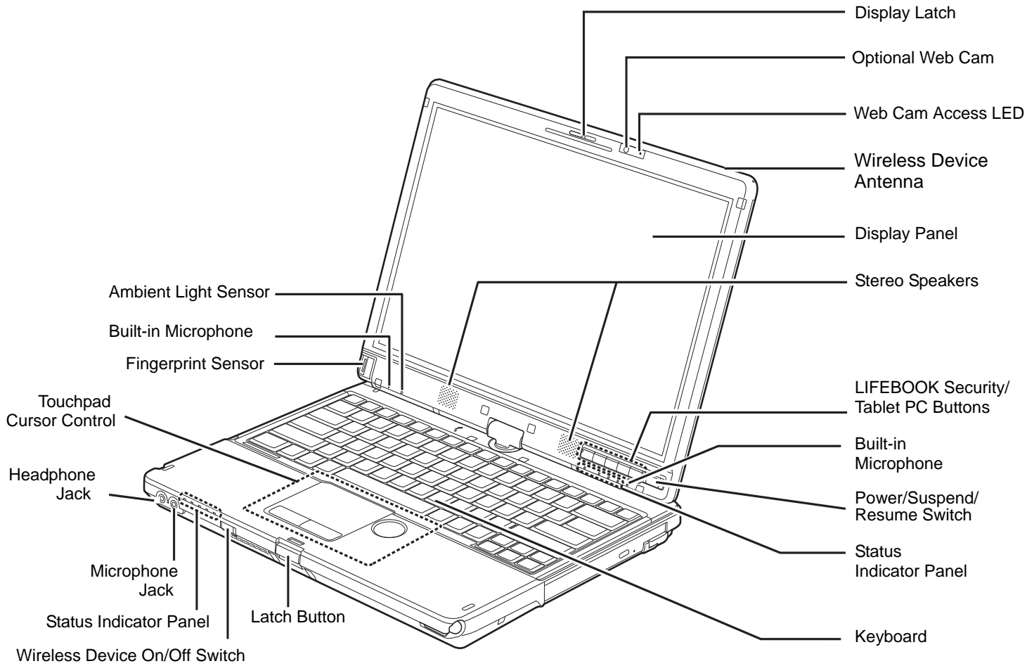
Figure 2. LIFEBOOK Tablet PC with display open
