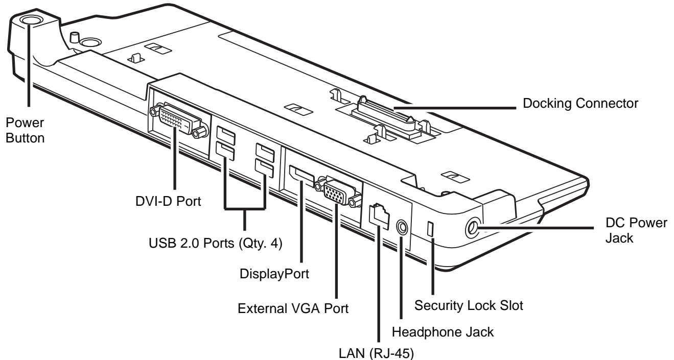
Figure 45. Port Replicator - Rear
