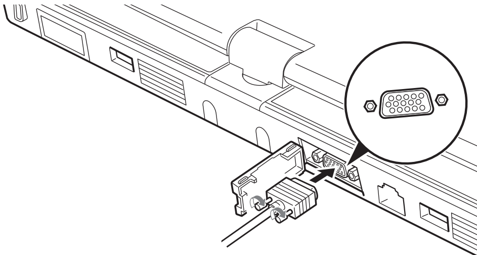
Figure 44. Connecting an External Video Device
