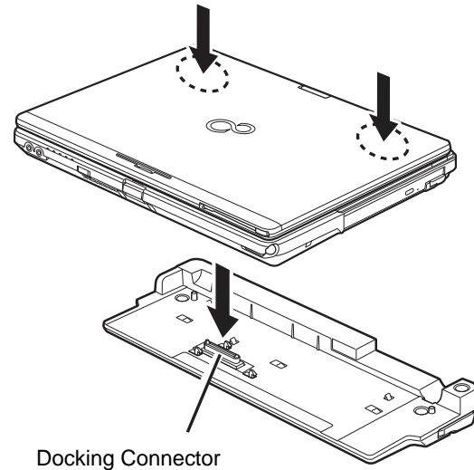
Figure 46. Attaching the Port Replicator
