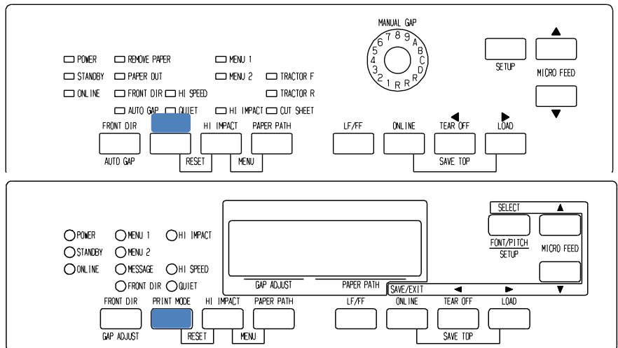
Print control panel
