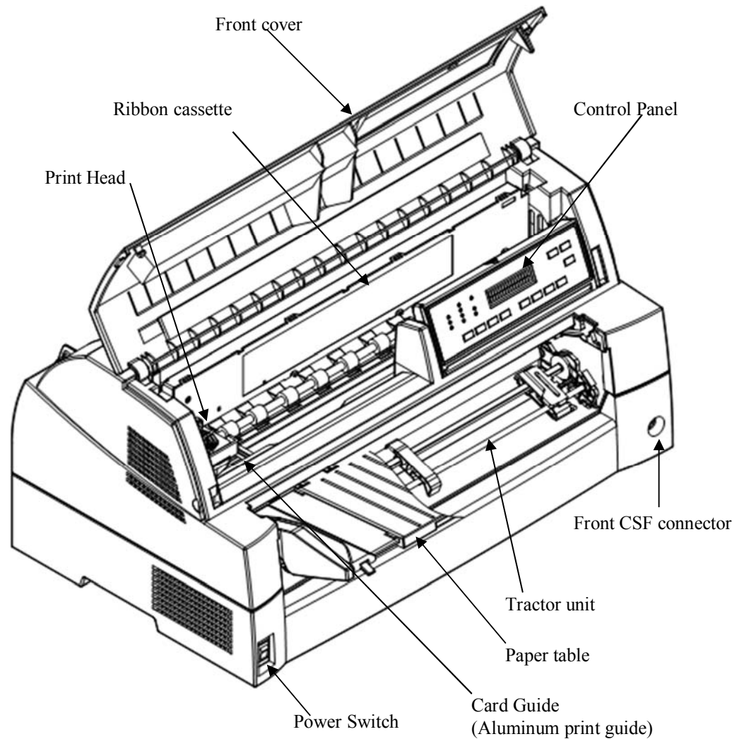
Printer components (front)
