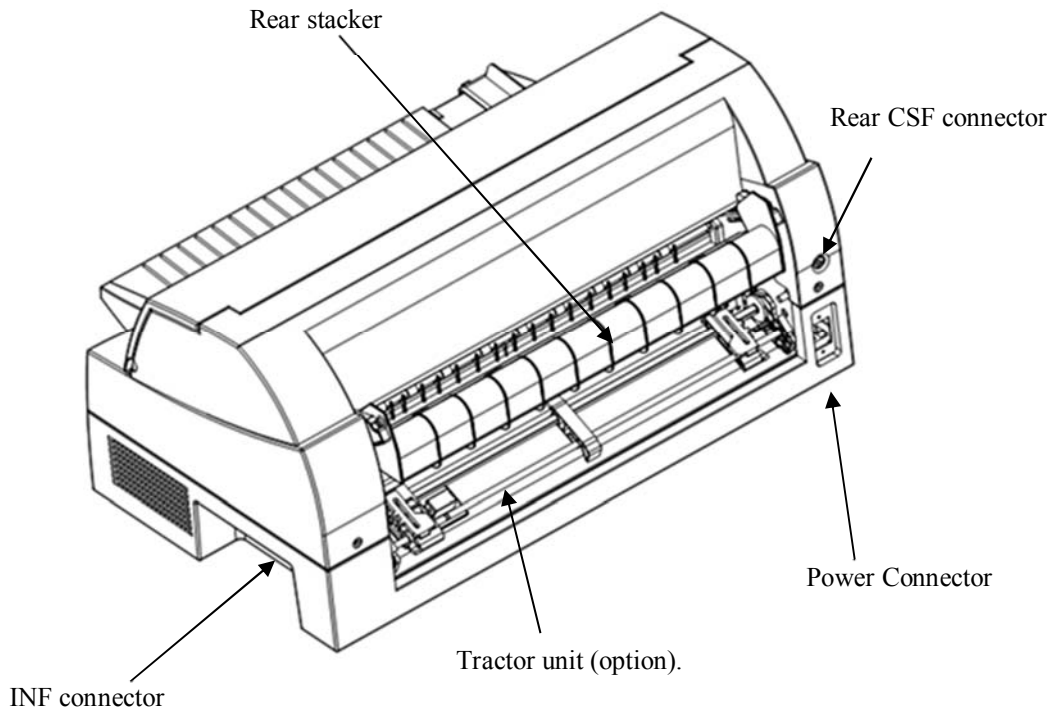
Printer components (rear)
