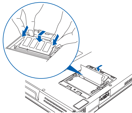
Figure 4-10. Installing a Second Memory Module
