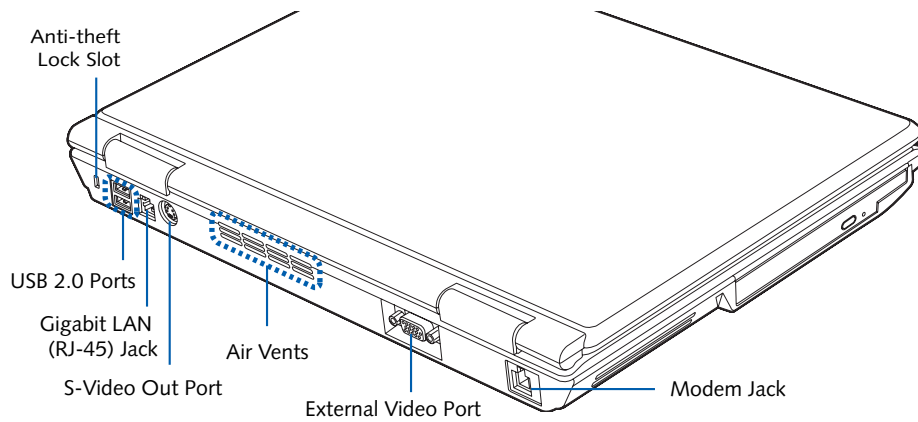
Figure 2-6. LifeBook notebook back panel
