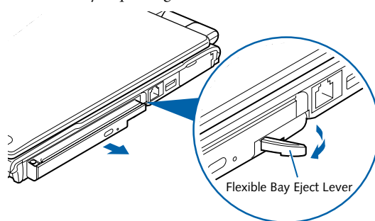
Figure 2-17 Removing/Installing a device in the Flexible Bay
