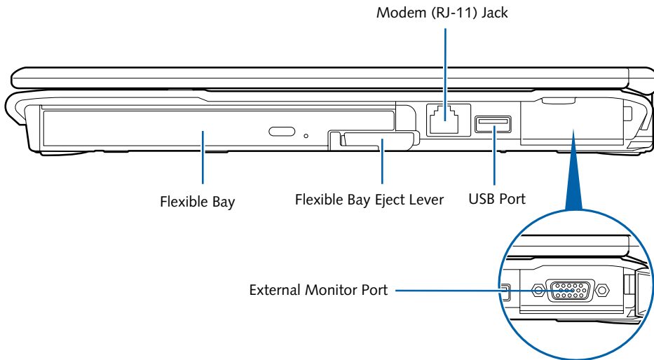
Figure 2-6. LifeBook notebook right-side panel
