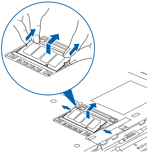
Figure 4-15. Removing a Memory Upgrade Module
