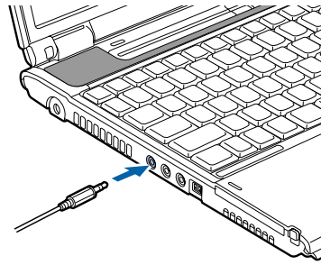
Figure 4-23. Connecting an S-Video Device
