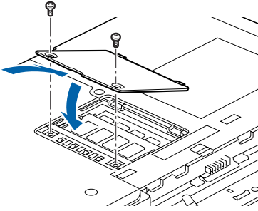
Figure 4-14. Replacing the Memory Compartment Cover
