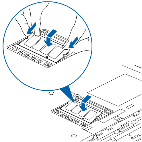
Figure 4-13. Installing a Second Memory Module
