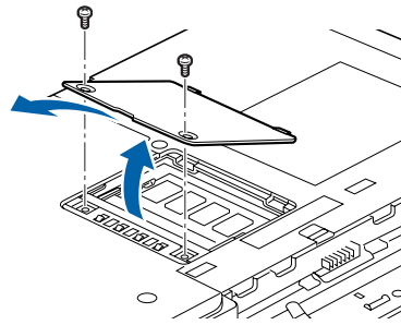
Figure 4-12. Opening the Memory Upgrade Compartment
