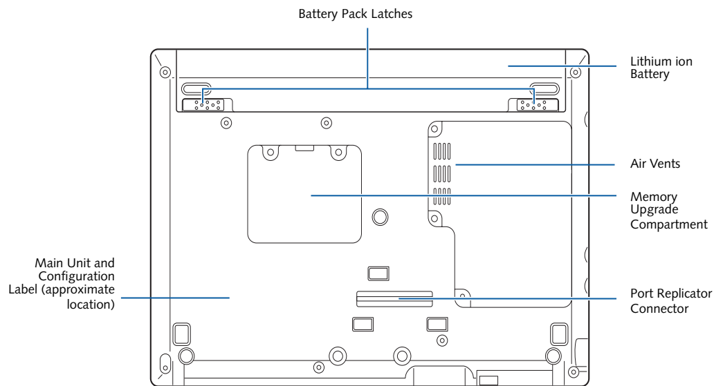
Figure 2-8. LifeBook P1600 Series notebook bottom panel
