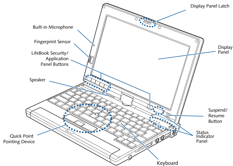
Figure 2-4. LifeBook P1600 Series notebook with display open
