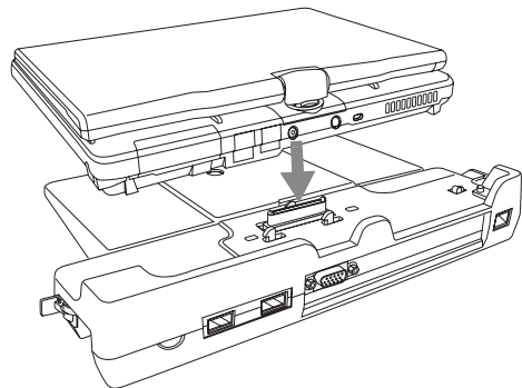
Figure 4-8. Attaching the Port Replicator
