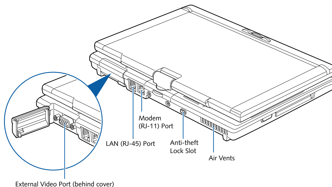
Figure 2-7. LifeBook P1600 Series notebook rear panel
