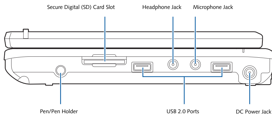
Figure 2-6. LifeBook P1600 Series notebook right-side panel
