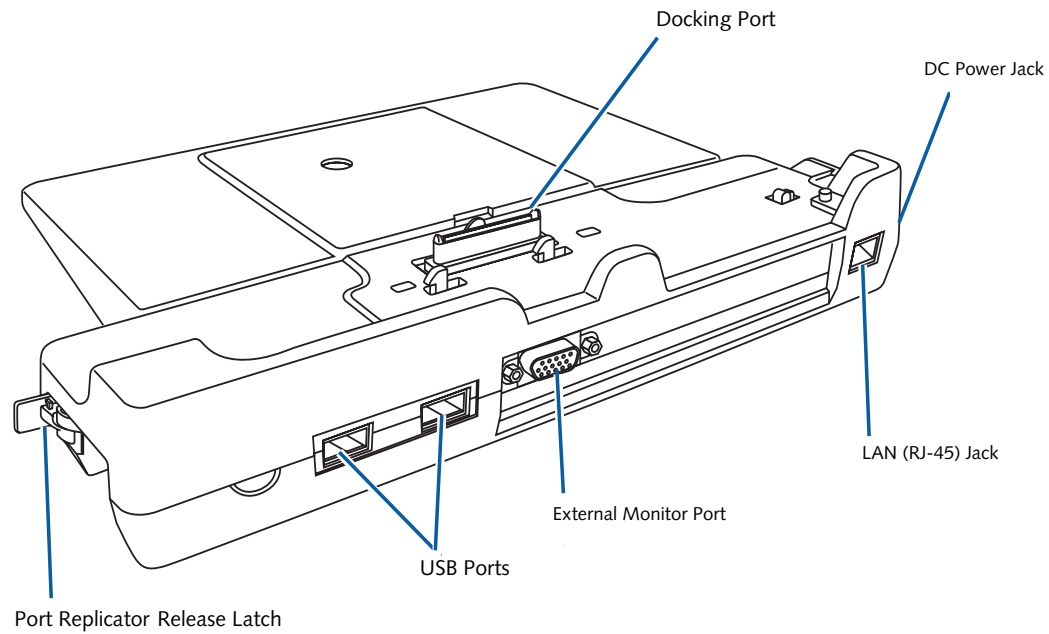
Figure 4-7. Port Replicator rear panel
