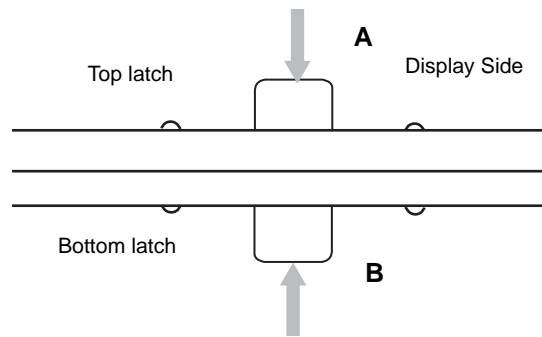
Figure 2-11. Using the Display Latch
