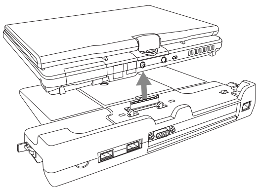
Figure 4-10. Removing the Port Replicator
