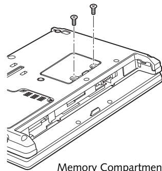
Memory Compartment Cover
