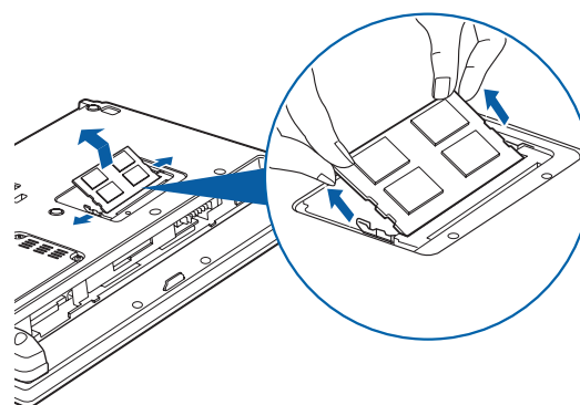
Figure 4-3. Removing a Memory Module
