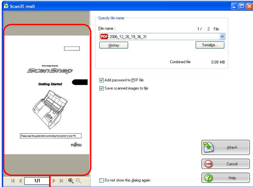
Preview Window
