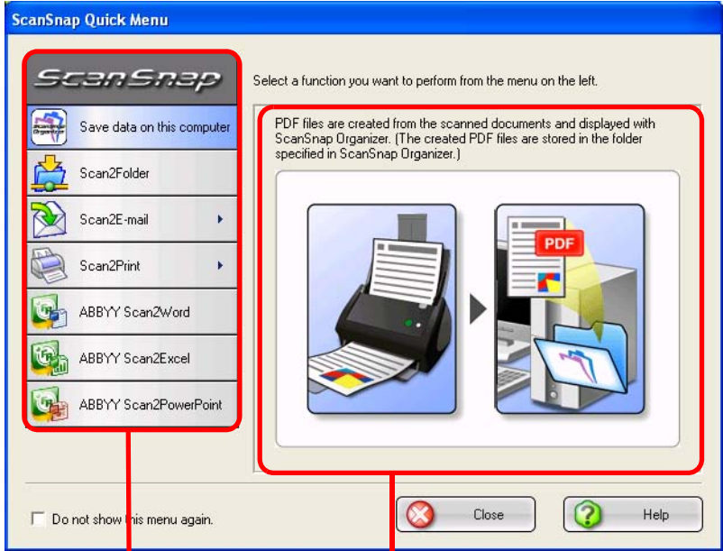
Action List
