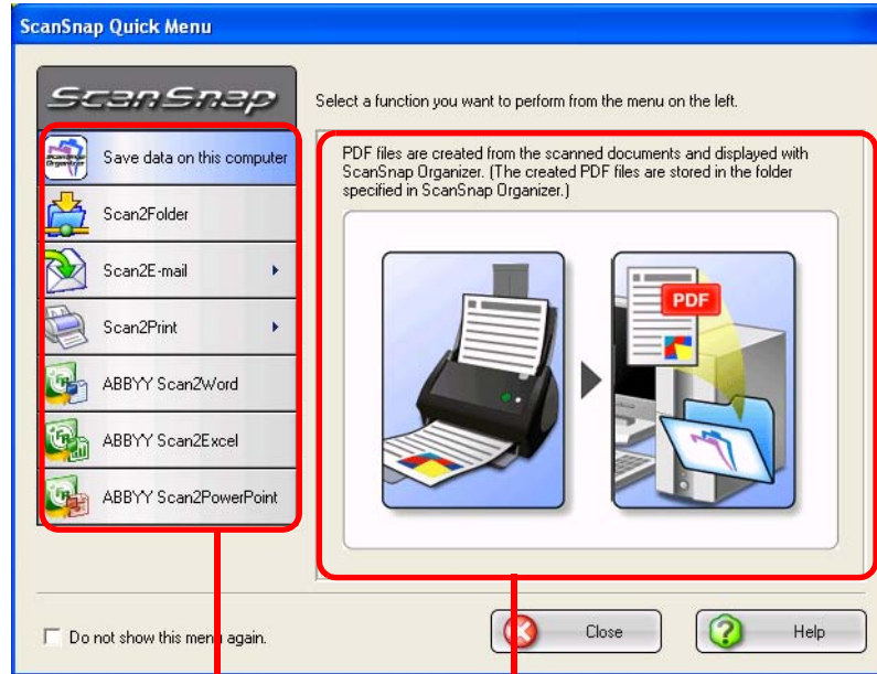
Action List
