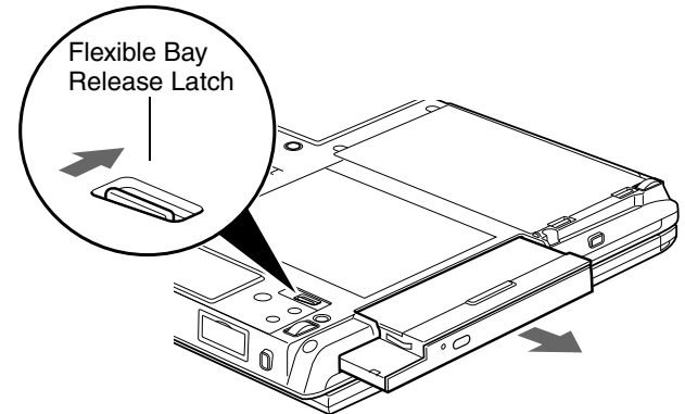
Figure 30. Removing/Installing Flexible Bay Device
