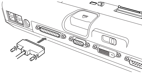
Figure 4-17. Connecting a Parallel Device to Port Replicator
