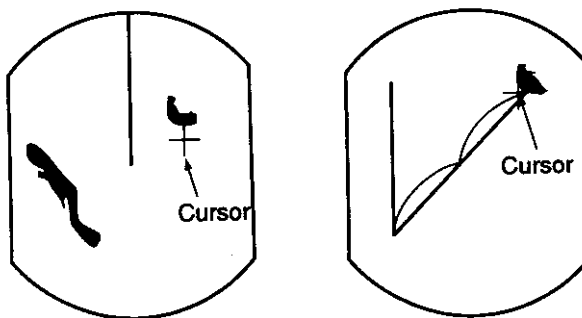
Figure 2-12 Measuring the range and bearing between two targets by using the offset EBL
