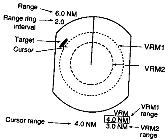
Figure 2-9 Measuring range by the cursor and VRM
