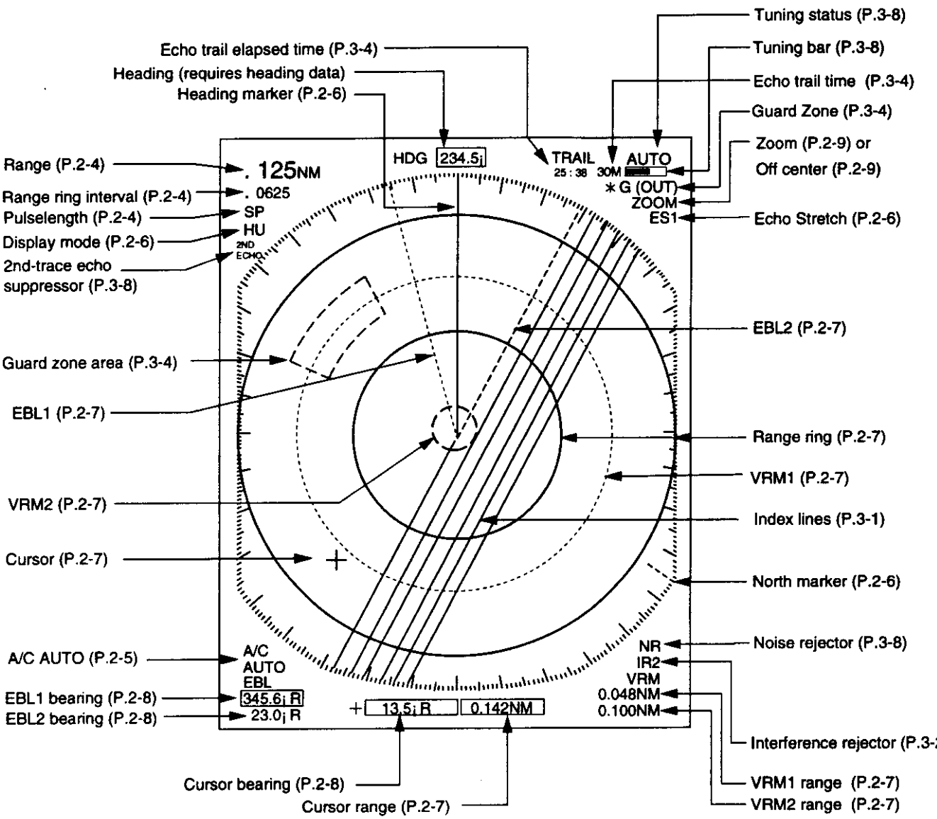
Figure 2-2 Display indications
