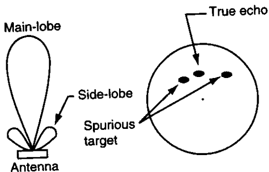
Figure 4-2 Side-lobe echoes
