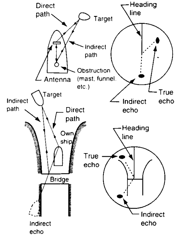
Figure 4-3 Indirect echoes
