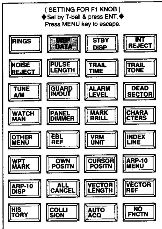
Figure 3-10 Function menu
