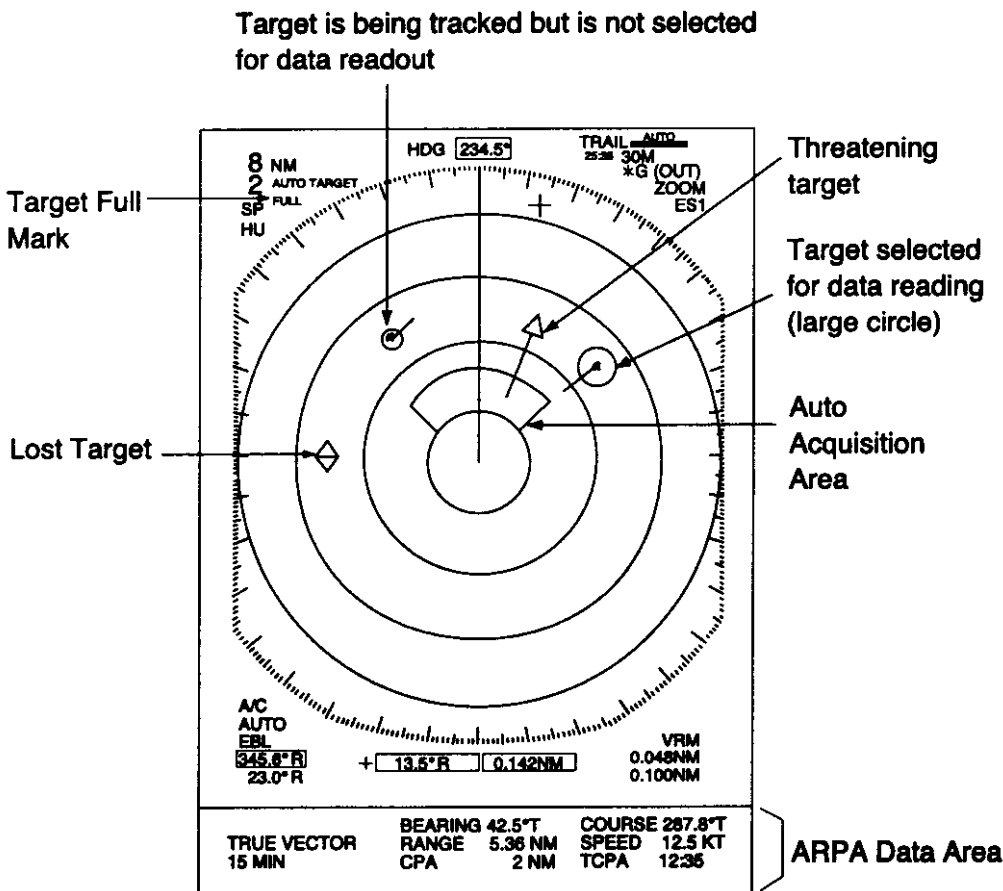
Figure 6-2 ARP display
