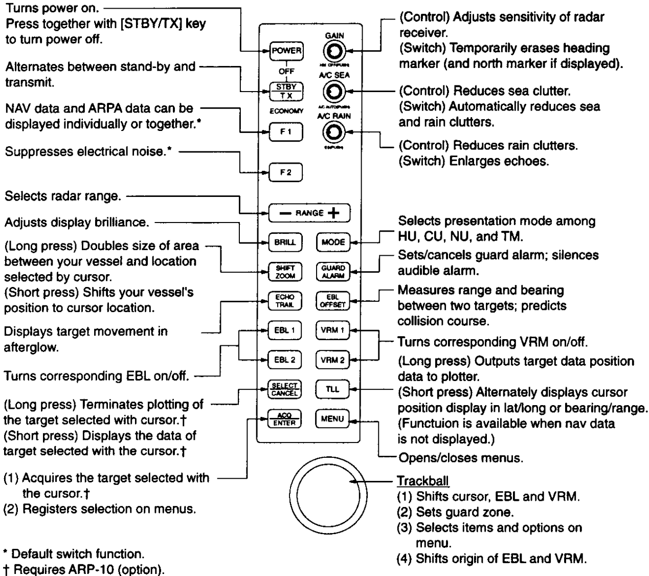
Figure 2-1 Control panel
