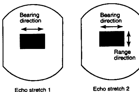
Figure 2-7 Echo stretch
