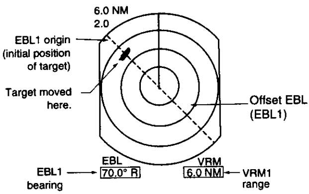
Figure 2-11 Predicting collision course by using the offset EBL
