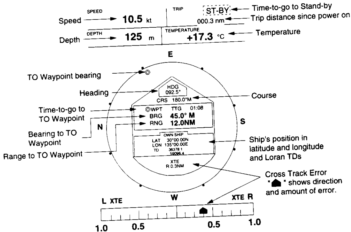
Figure 2-3 Typical navigation data display during stand-by
