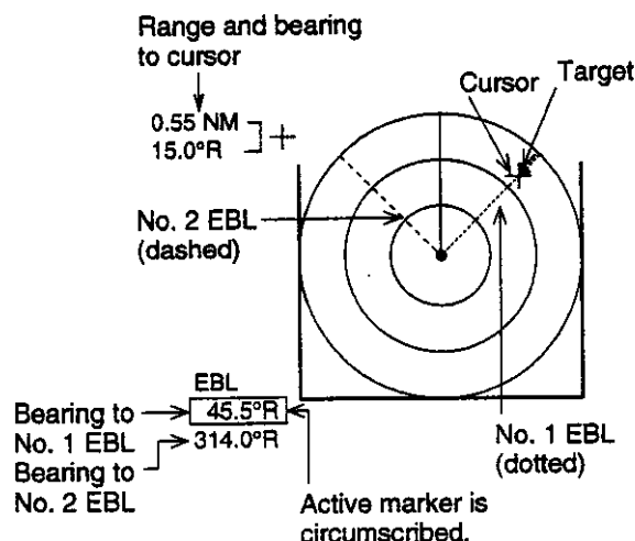
Figure 1-16 How to measure bearing by EBL
