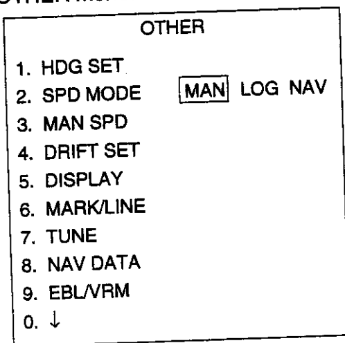
Figure 2-7 OTHER menu
