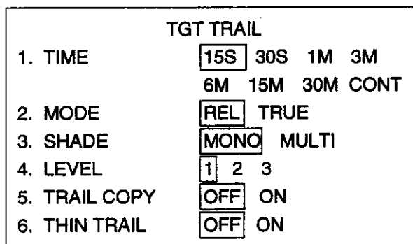
Figure 1-32 TGT TRAIL menu
