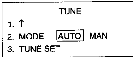
Figure 1-6 TUNE menu
