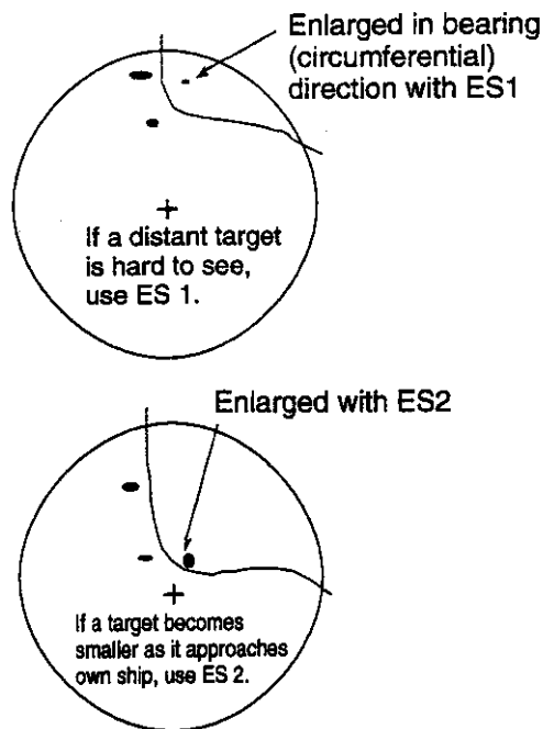
Figure 1-10 Echo stretch
