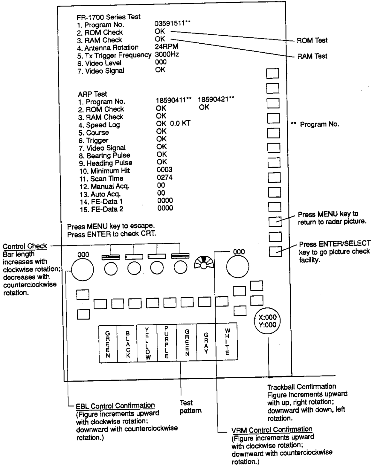
Figure 3-2 Test results screen
