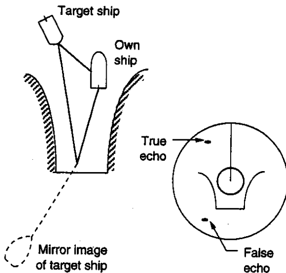
Figure 2-4 Virtual image
