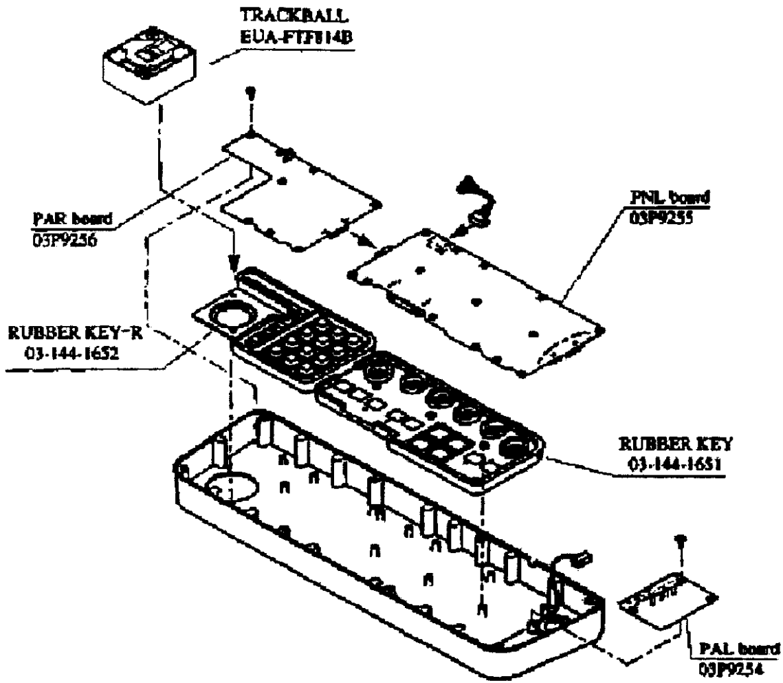
EXPLODED VIEW OF DISPLAY UNIT CONTROL HEAD
