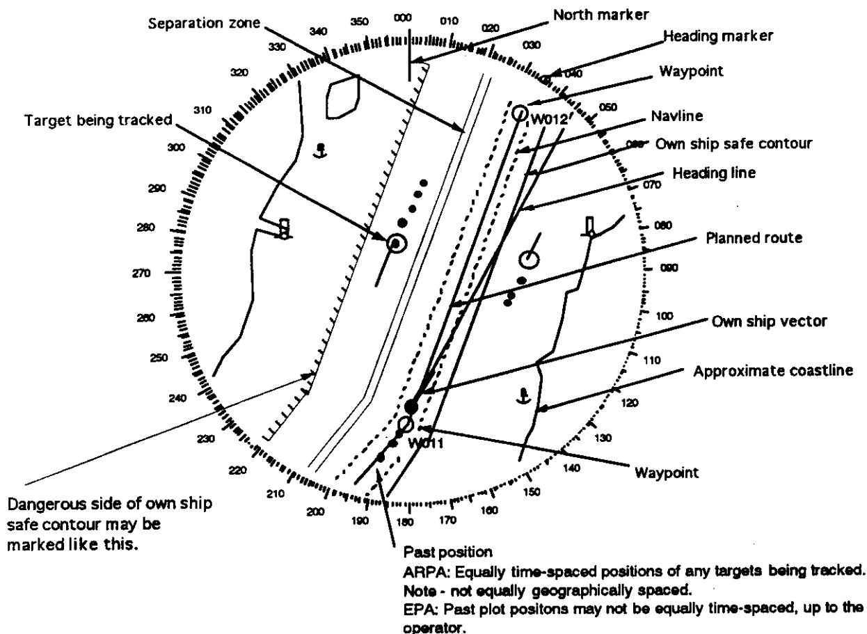
Concept of Radar map, Ground stabilized
