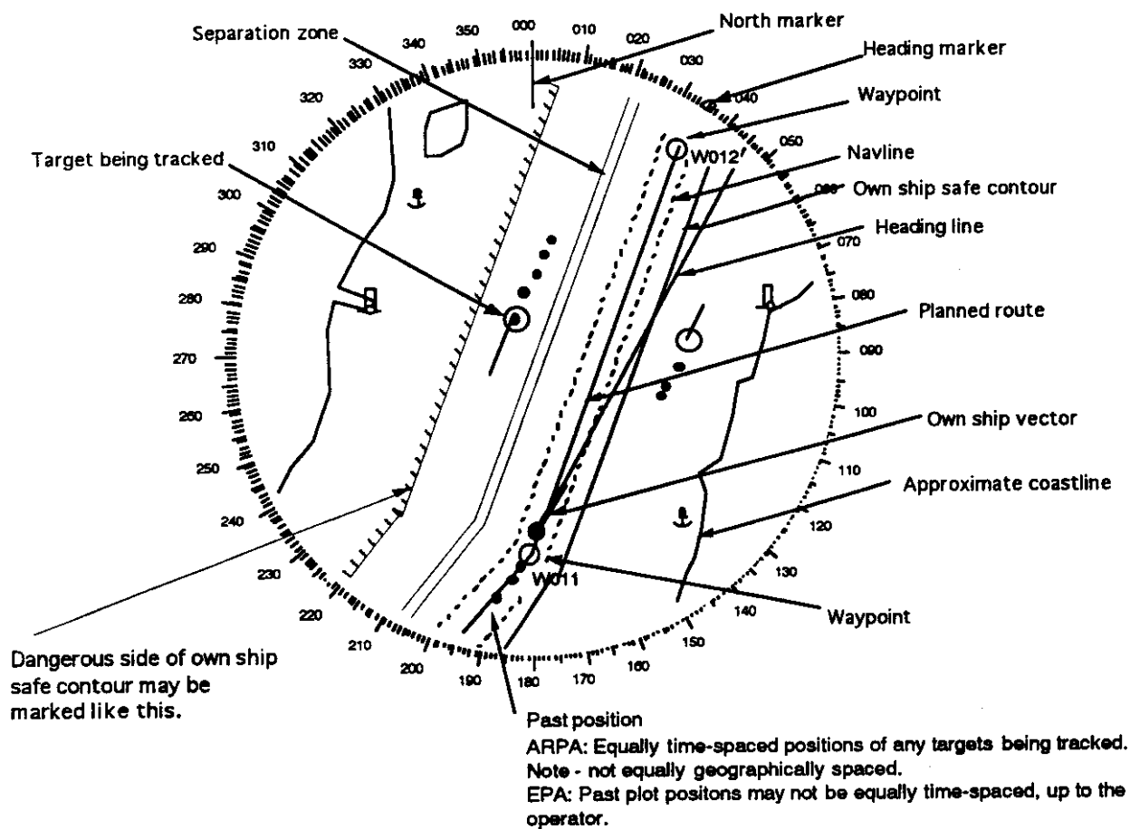
Concept of Radar map, Ground stabilized (Above excludes radar pictures. In reality, radar echoes are always displayed)
