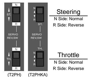
(Reversing Switches)
