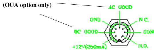
Alarm/Optional Power Supply Pinout (Relay States Refer To NON Alarm Condition)
