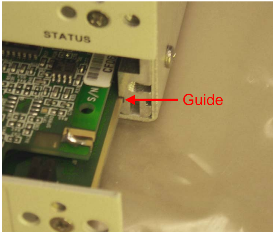
Figure 3-17 Guides
