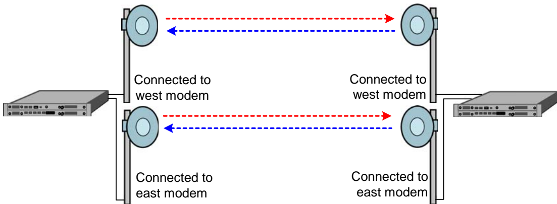
Figure 2-9. 1+1 protection in diversity mode
