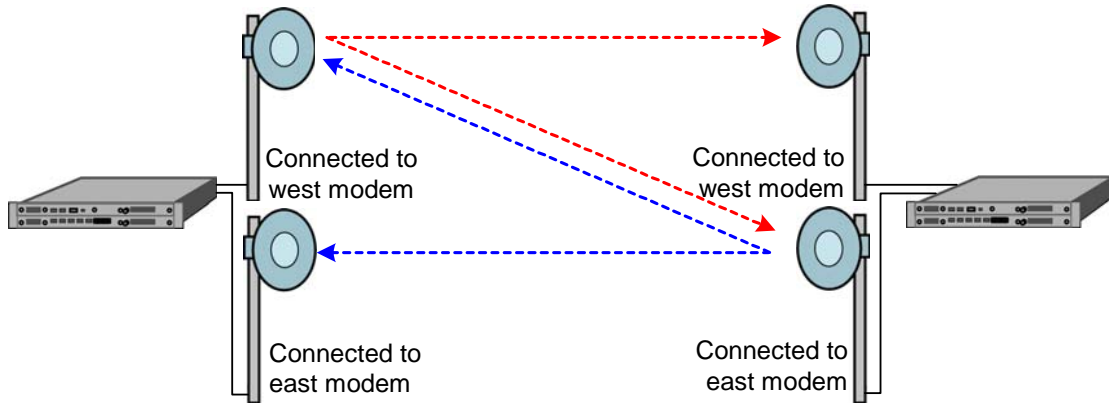
Figure 2-8. 1+1 protection in non-diversity mode
