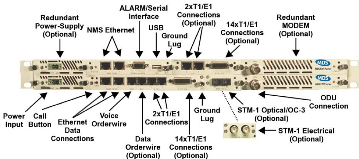
Figure 2-3. SDIDU™ Front Panel Connections
