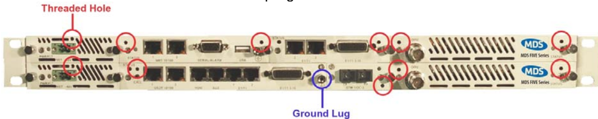
Figure 3-16 Threaded Hole Locations
