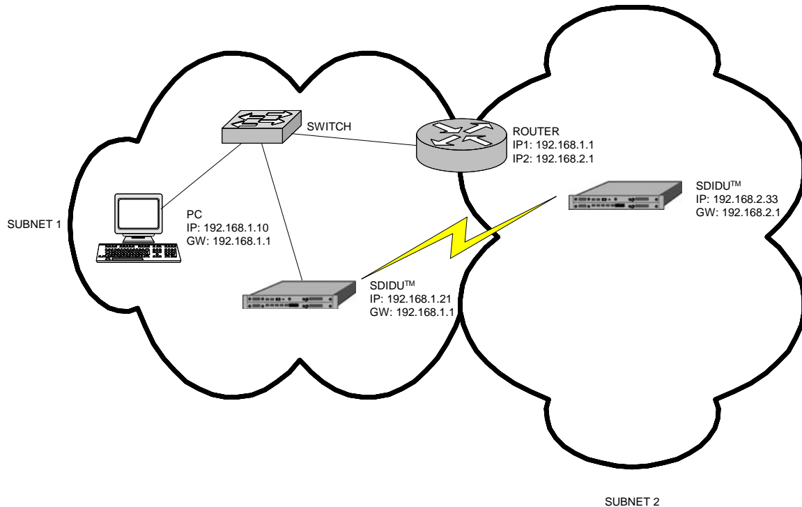
Figure 2-15. SDIDUs™ on different subnets.
