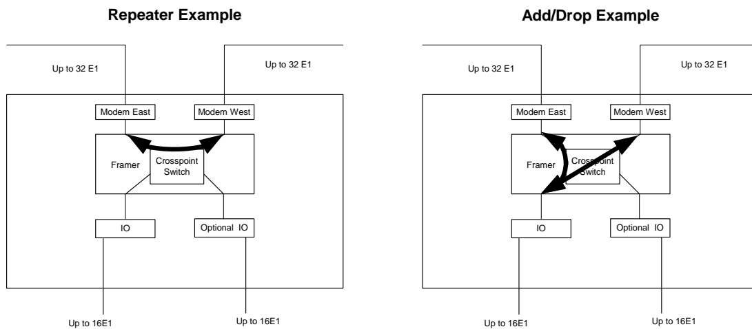
Figure 2-12 Crosspoint switch
