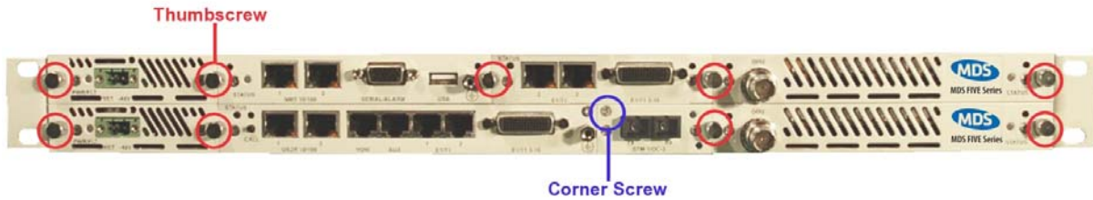
Figure 3-15 Thumbscrew and Corner Screw Locations
