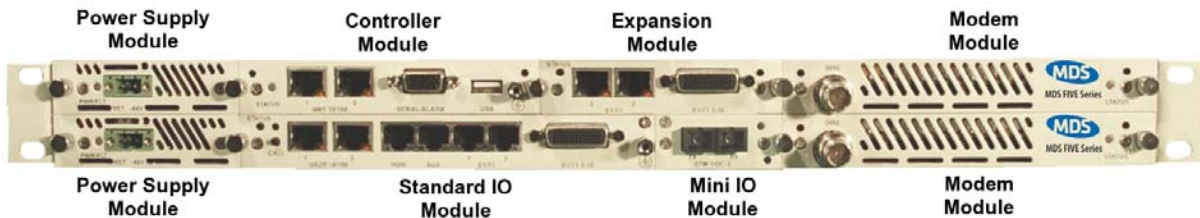
Figure 3-14 SDIDU™ Modules
