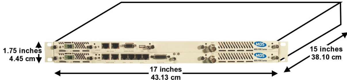
Figure 3-5. MDS FIVE Series SDIDU™ Dimensions
