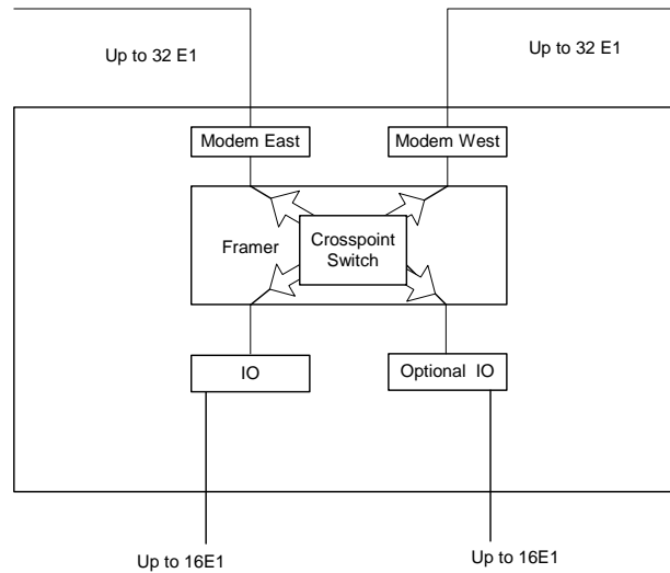
Figure 2-12 Crosspoint switch
