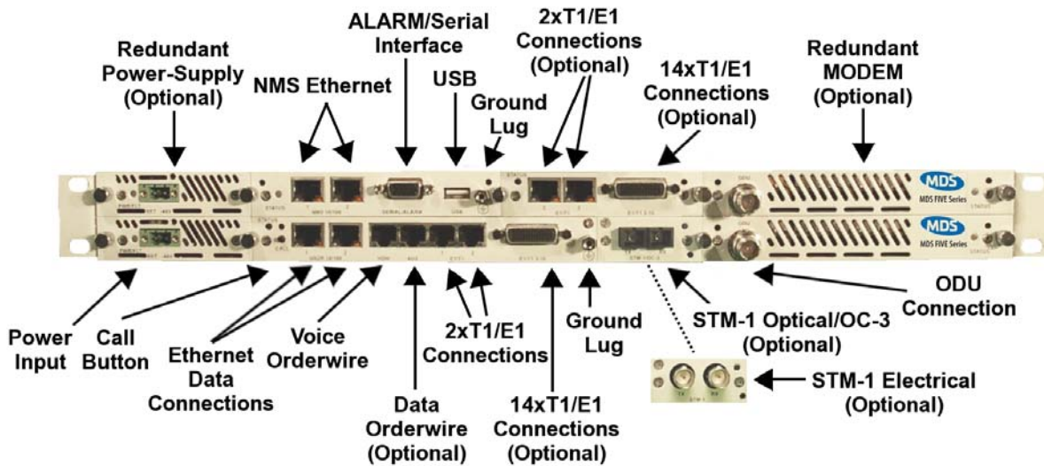
Figure 3-12. MDS FIVE Series-SB, 1+1 Protection: SDIDU™ Front Panel Connections
