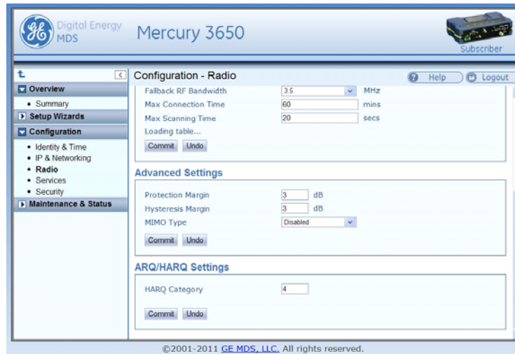
Figure 10. Configuration—Radio (HARQ Category Setting)
