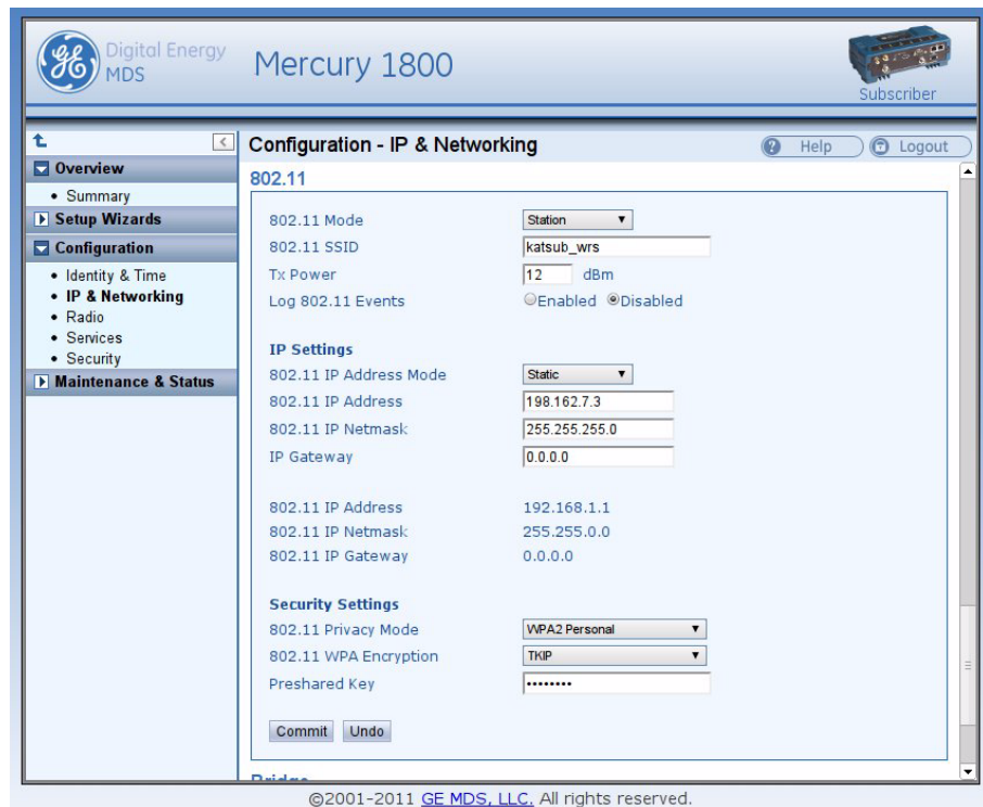
Figure 23. 802.11 Configuration for Station Mode
