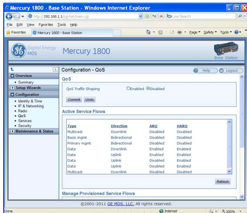
Figure 17. Configuration-QoS Screen (Active Service Flows)
