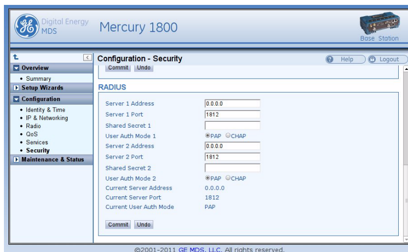
Figure 30. Configuration - Security Screen (RADIUS Portion)
