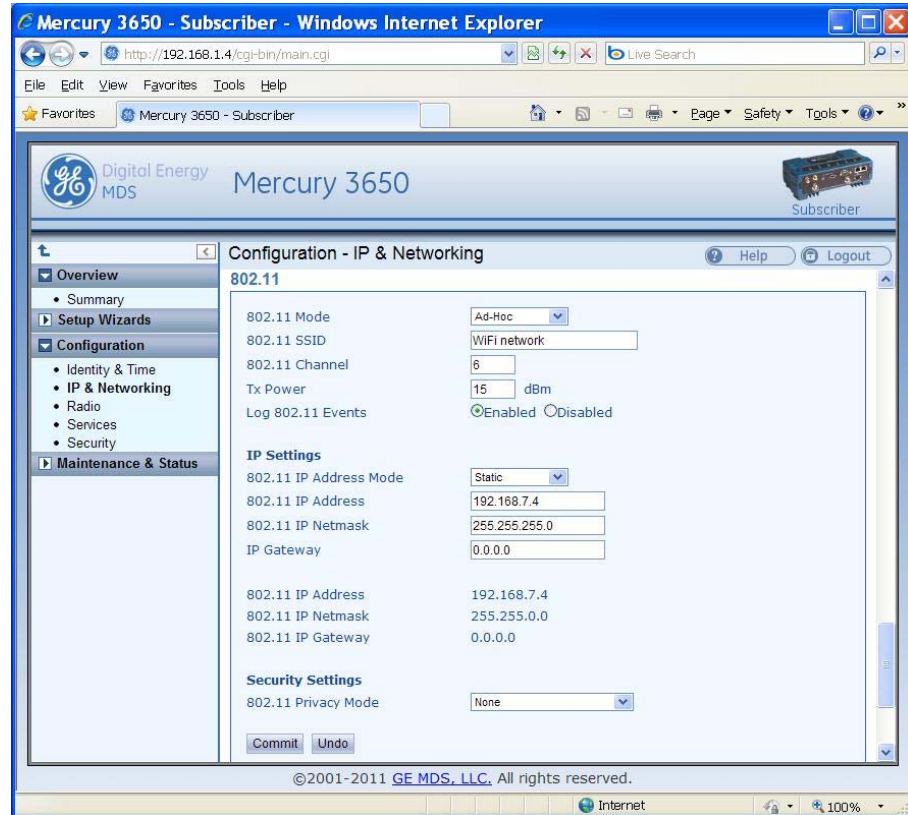
Figure 24. 802.11 Configuration for Ad-Hoc Mode
