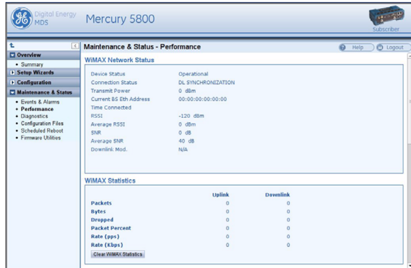
Figure 8. Maintenance and Status Screen
