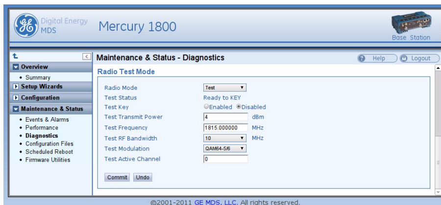
Figure 28. Radio Test Mode Screen
