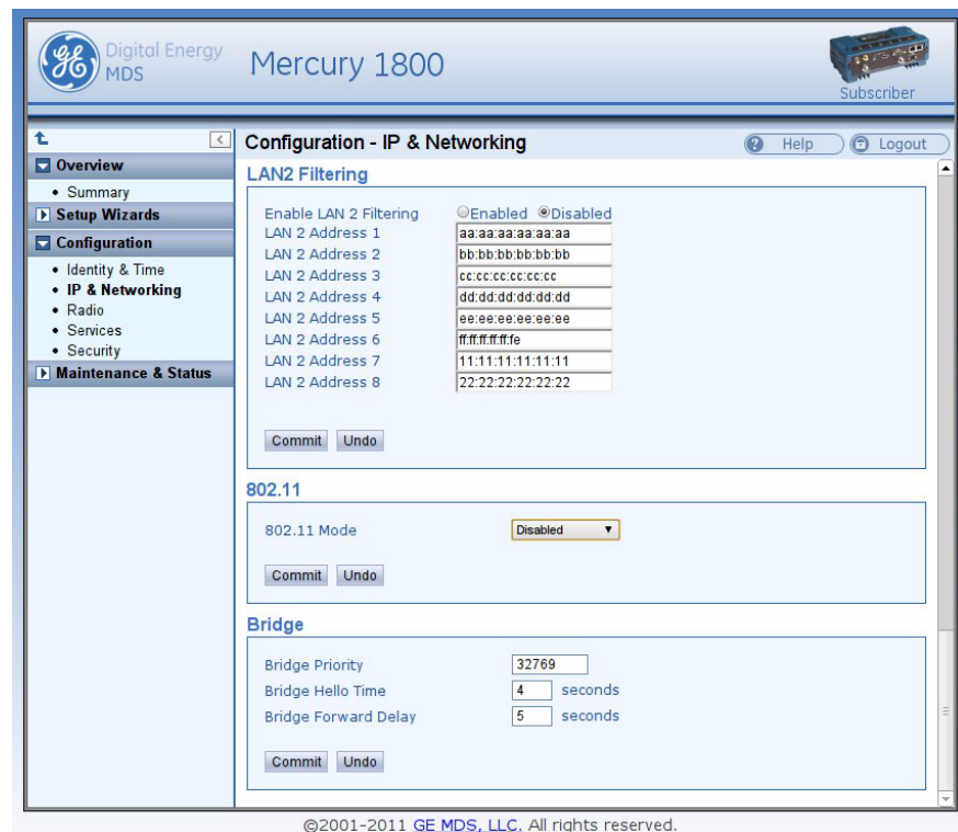
Figure 22. 802.11 Configuration (Default Screen)
