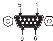
Figure 35. COM1 Port (DCE) (Viewed from the outside of the unit.)
