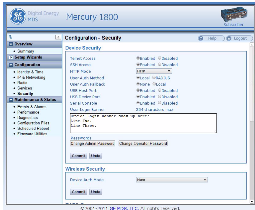
Figure 29. Configuration - Security Screen (Upper Portion)
