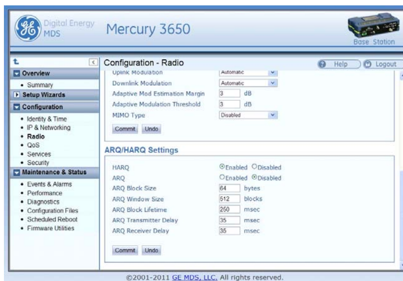
Figure 9. Configuration—Radio (ARQ/HARQ Settings)
