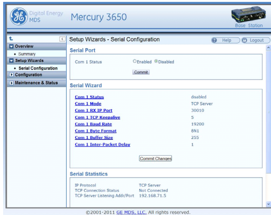
Figure 16. Serial Wizard's Commit Changes Screen
