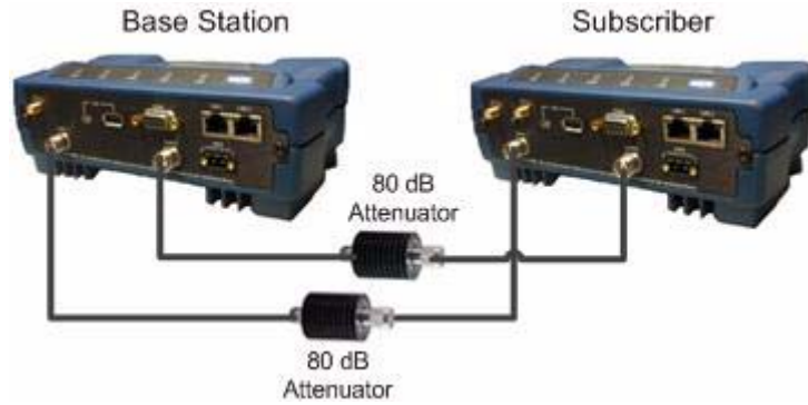
Figure 7. Benchtop Test Setup
