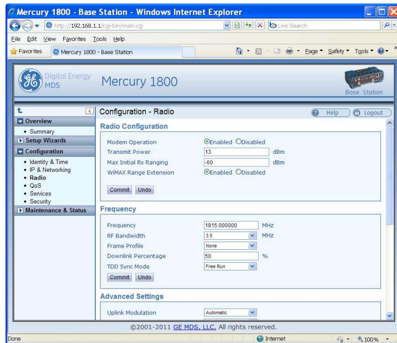
Figure 6. Mercury Configuration—Radio
