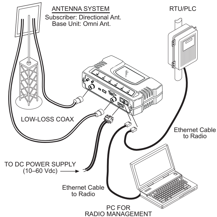
Figure 32. Typical Installation with a Tower-Mounted Antenna (SU shown; BS Similar)
