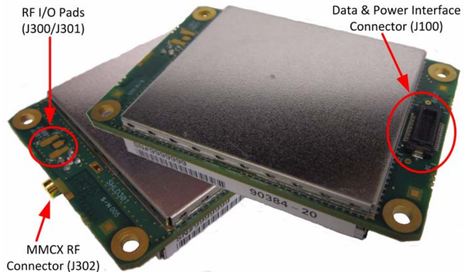
Figure 4. Transceiver Views Showing External Connections
