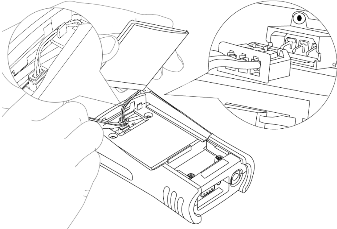
< Figure 4. Rechargeable Battery Installation >
