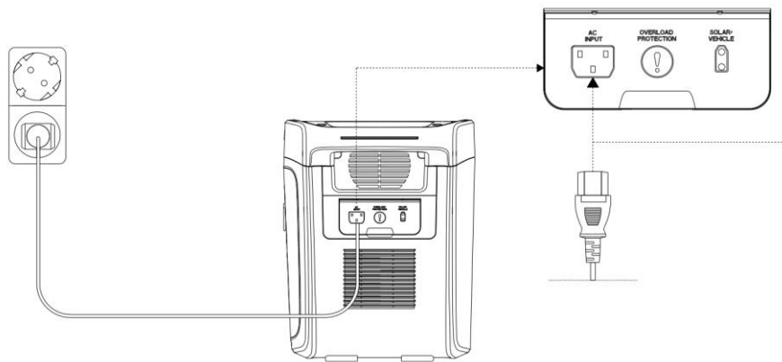
AC Charging
