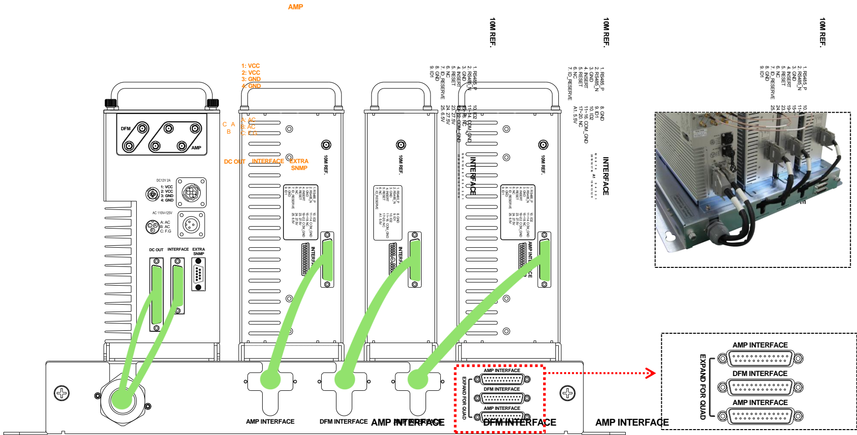
<Picture 9> Bottom View of the Repeater.
