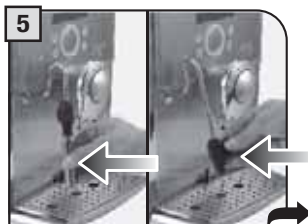
Remove the end part of the steam spout; remove and wash the steam spout support. Then reinsert it.
