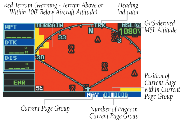
Figure 2-26 TERRAIN Page 120° View
