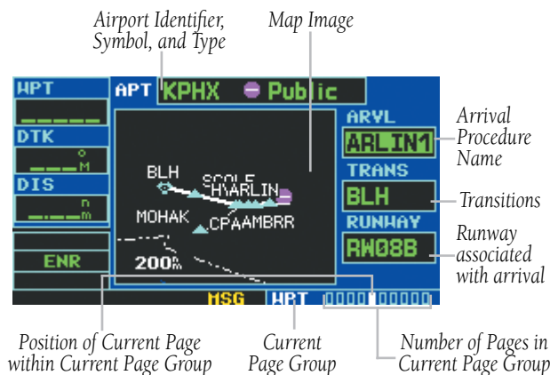
Figure 6-21 Airport Arrival Page
