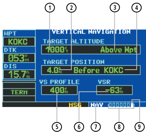
Figure 2-49 VNAV (Vertical Navigation) Page
