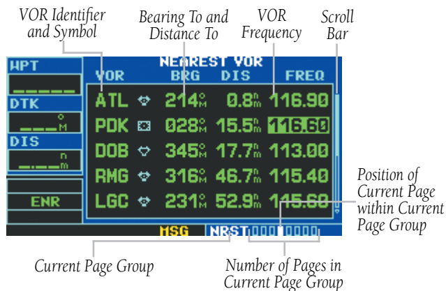
Figure 7-14 Nearest VOR Page
