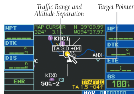
Figure 10-19 Traffic Range and Altitude Separation
