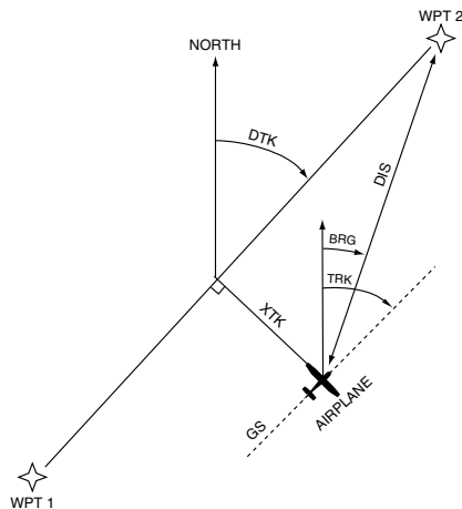
Figure 12-1 Illustrated NAV Terms
