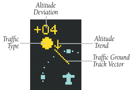
Figure 10-4 Traffic Symbol Components
