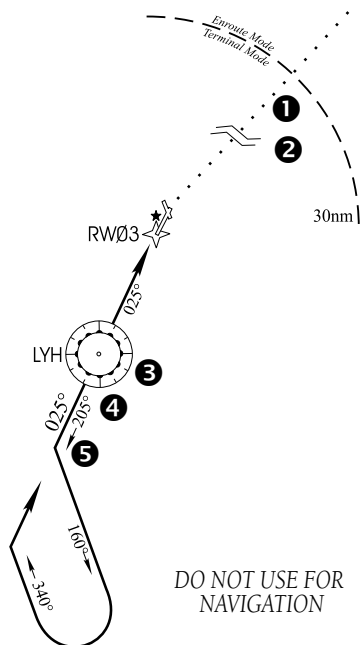
Figure 5-13 Sample Approach with Procedure Turn
