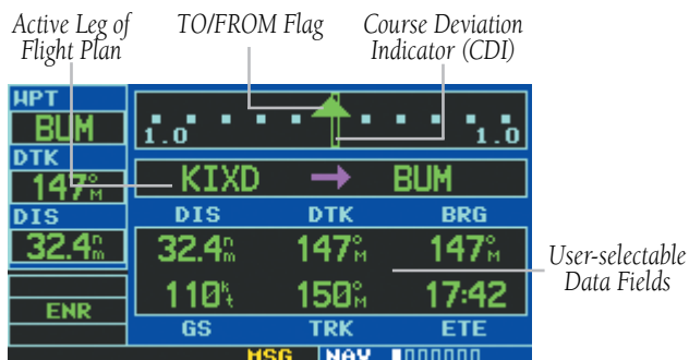
Figure 1-16 Default NAV Page
