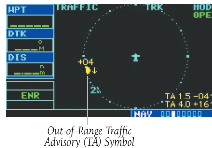
Figure 10-3 Out-of Range TA Symbol
