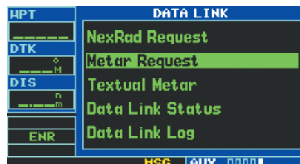
Figure 10-42 Data Link Page
