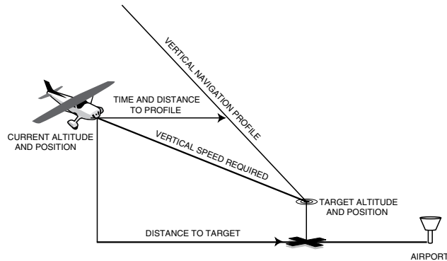
Figure 12-2 Illustrated Vertical NAV Terms
