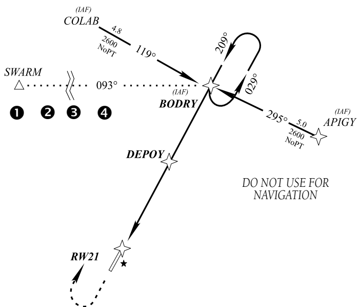
Figure 5-25 Approach with Hold
