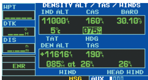
Figure 8-19 Heading Field Highlighted
