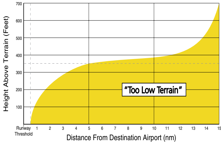
Figure 9-5 PDA Alerting Threshold
