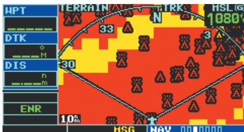
Figure 2-29 TERRAIN Display Range
