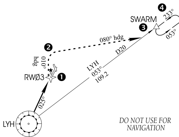
Figure 5-21 Sequence to MAP
