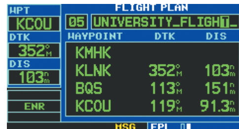
Figure 4-8 Comment Line Selected
