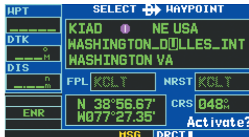
Figure 3-5 Facility Name Selected
