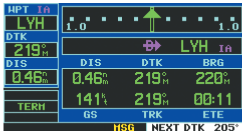
Figure C-6 CDI at 1 nm Scale
