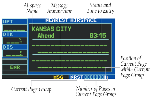
Figure 7-21 Nearest Airspace Page
