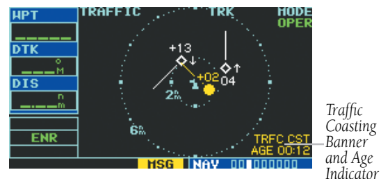
Figure 10-6 Traffic Age Indicator and Coasting Banner
