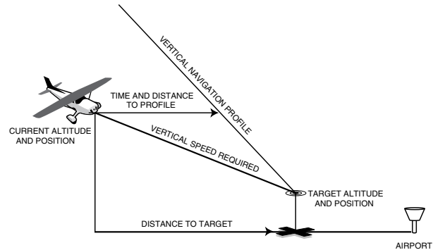
Figure 2-50 Vertical Navigation Profile
