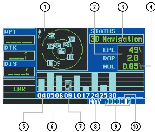
Figure 2-47 Satellite Status Page
