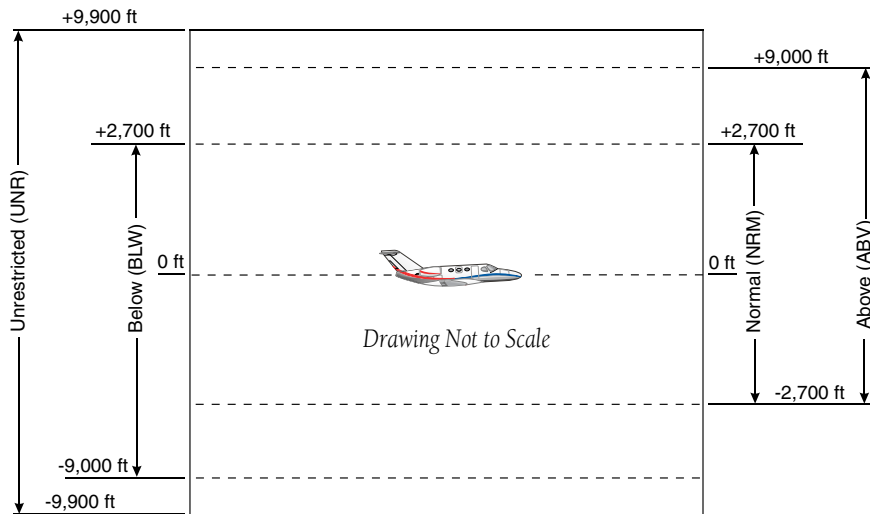
Figure 10-24 Altitude Display Modes
