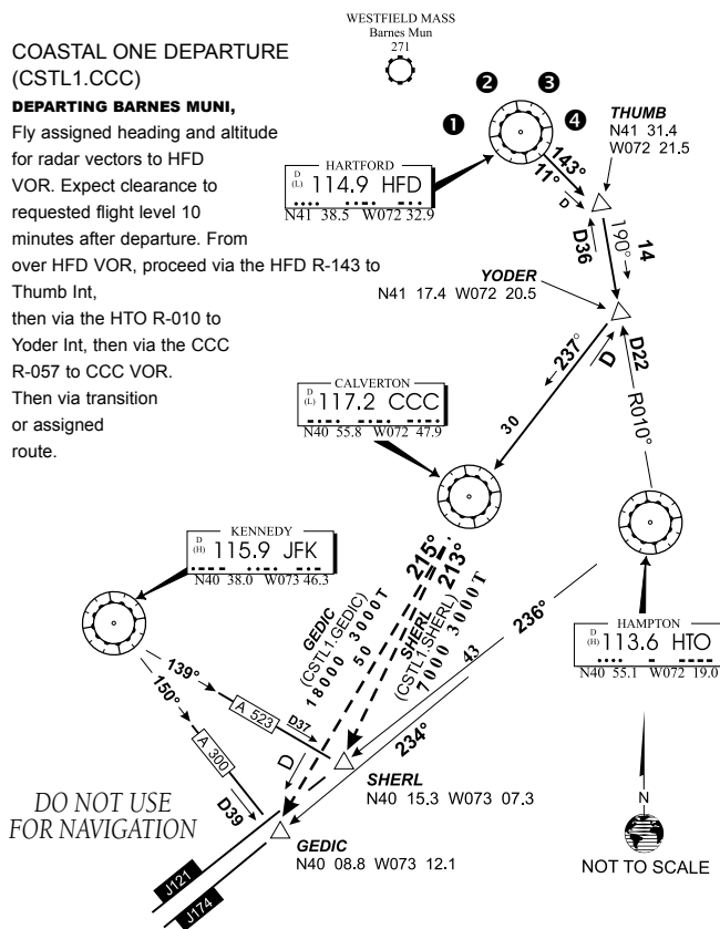
Figure 5-69 Coastal One Departure
