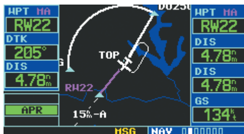
Figure 5-47 Final Course Segment
