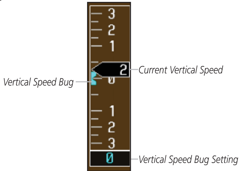
Vertical Speed
