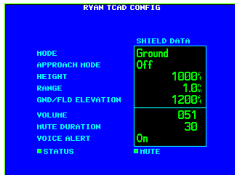
Figure 5-19. RYAN TCAD CONFIG Page
