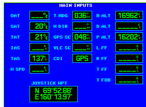
Figure 5-3. MAIN INPUTS Page
