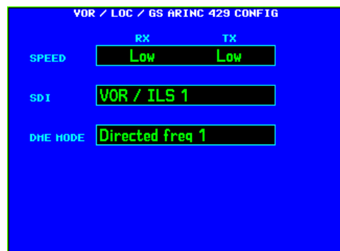
Figure 5-13. VOR/LOC/GS ARINC 429 CONFIG Page
