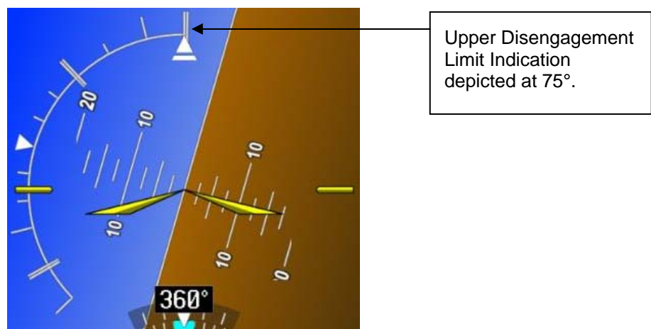
Figure 14 – Minimum and Maximum Roll Attitude ESP Disengagement Limit Indications
