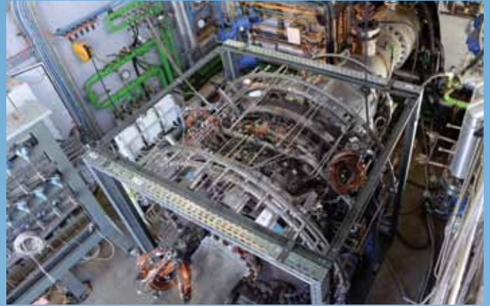
Full scale combustion vessel for full-annular-rig test
