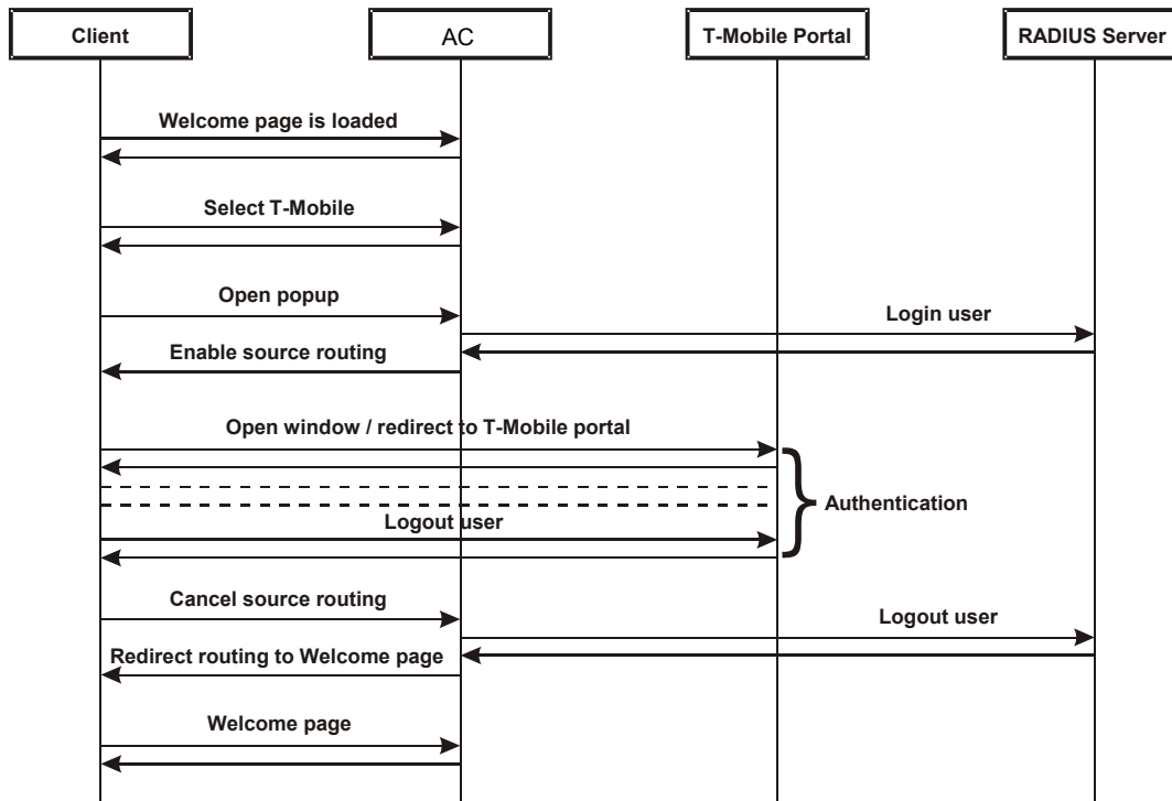
Figure 106 – One-Click Roaming diagram
