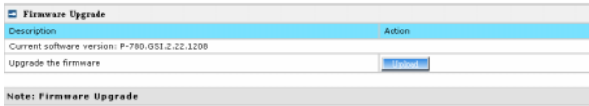
Figure 62 – Firmware Upgrade
