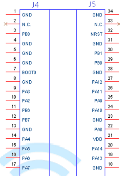
FIGURE 1-2: GL6509 PIN HEADER PIN DIAGRAM(Top View)
